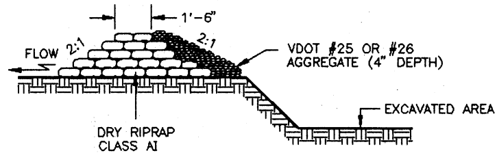
CROSS-SECTION B-B
